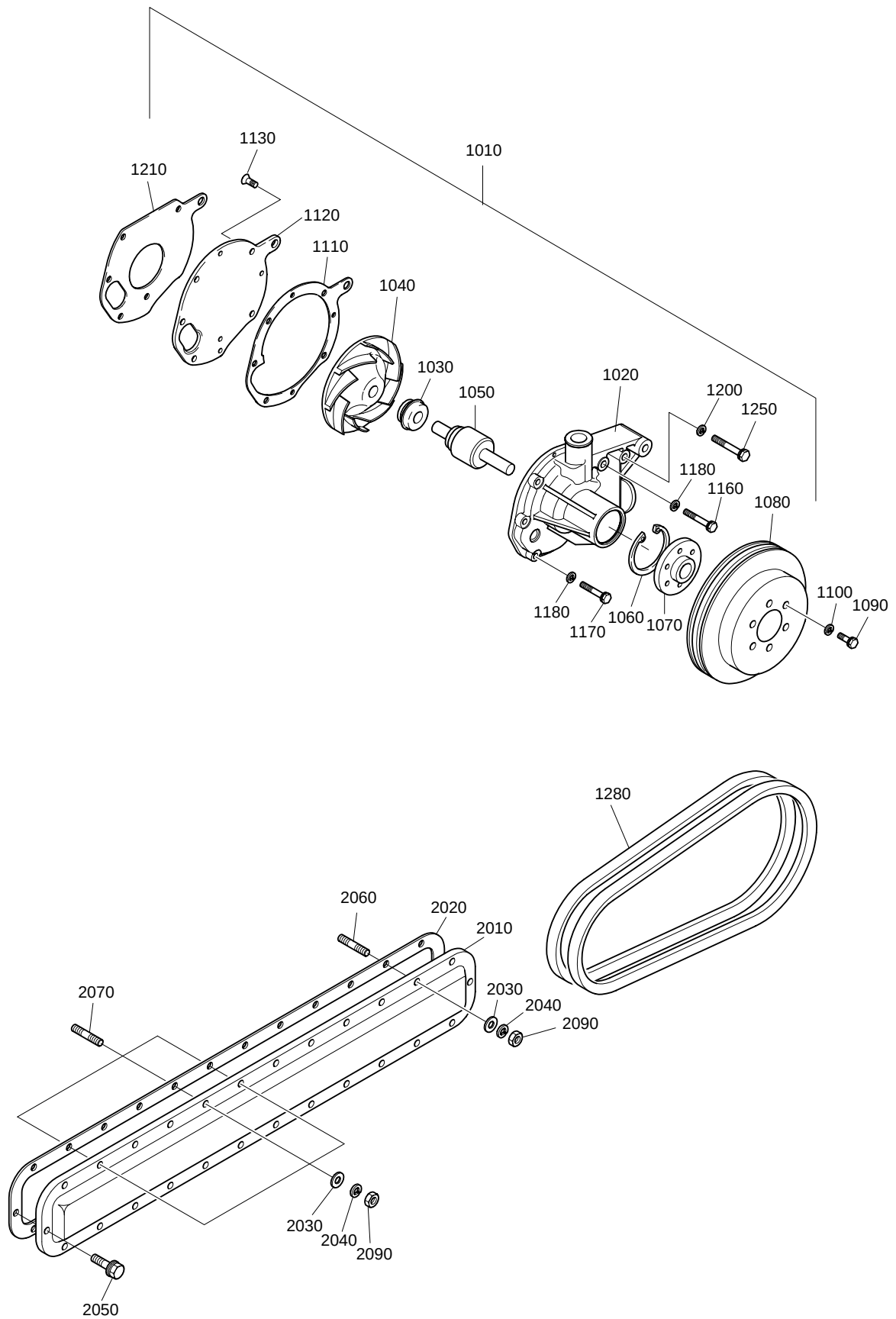
냉각수 펌프 Fig.013 COOLING WATER PUMP
